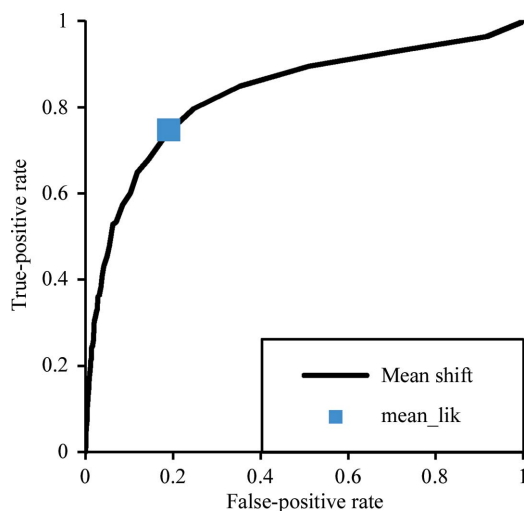
Figure 4 ROC curve for the decision-making procedure based on the mean shift. The curve corresponds to the class of ‘side inner’ residues (test sample, database 1, 0.0961 \leq R_{work} \leq 0.1278 ). The square marker shows the quality of the procedure based on the likelihood of the mean shift (mean_lik).
